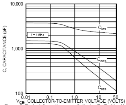
Figure 5, Typical Capacitance vs Collector-To-Emitter Voltage
