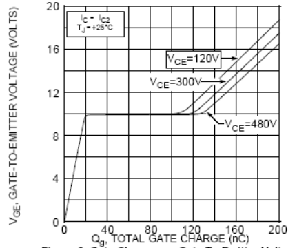
Figure 6, Gate Charges vs Gate-To-Emitter Voltage
