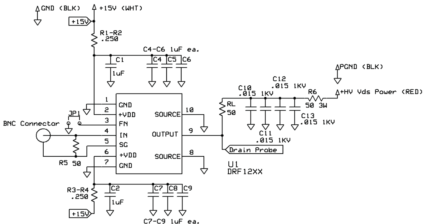
Figure 2, DRF1201 Test Circuit
