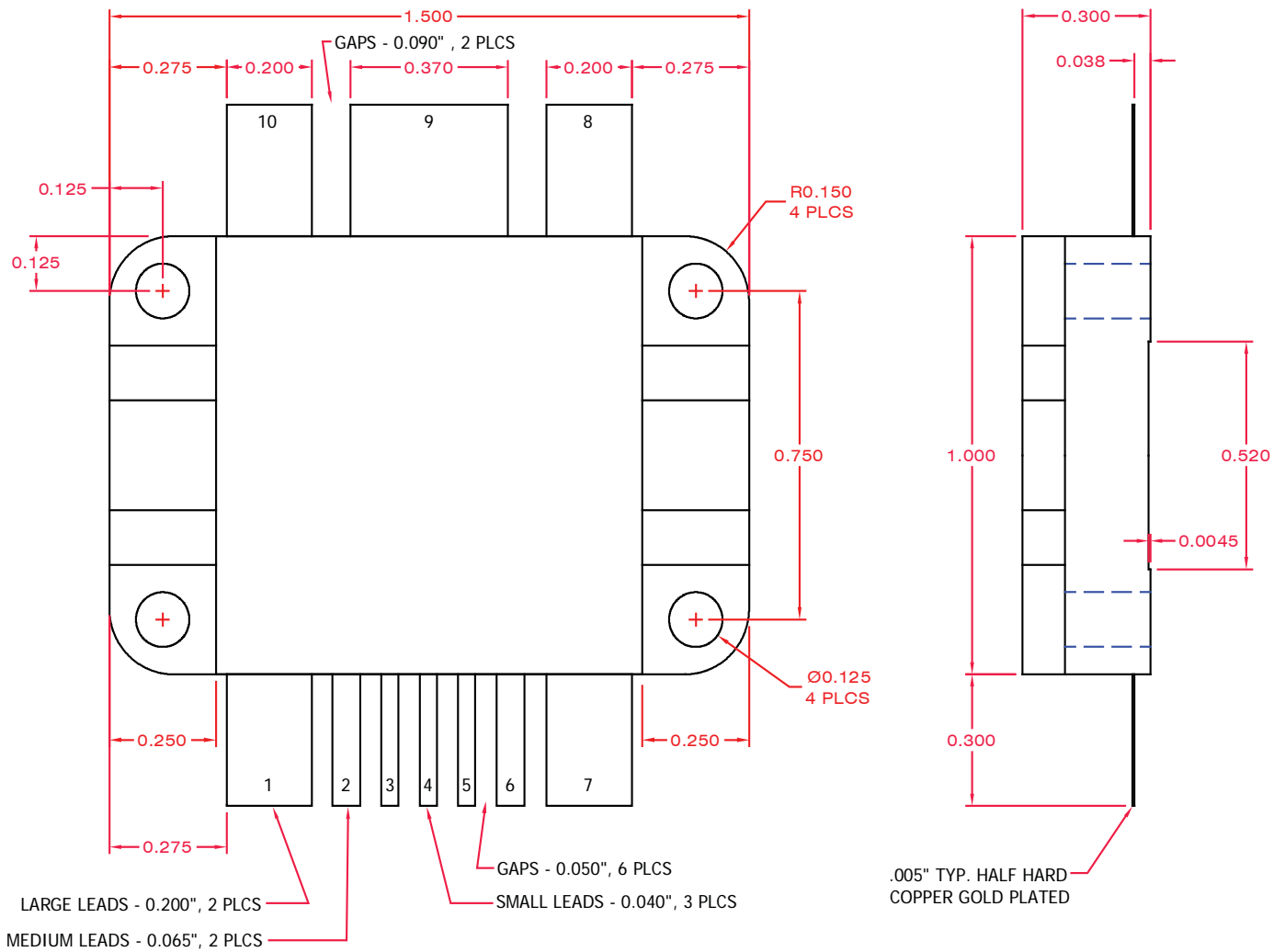
Figure 3, DRF1201 Mechanical Outline
