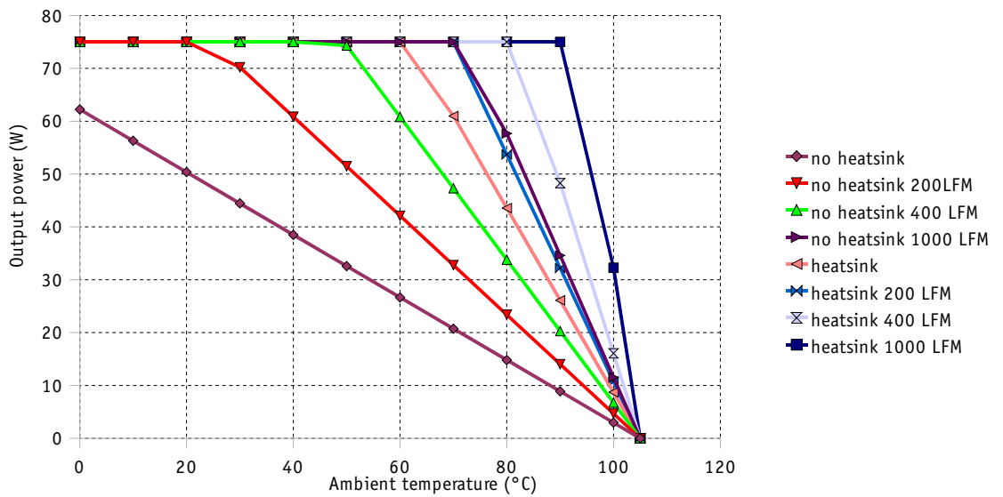
MGDS-75-O-x Series Thermal Curves
