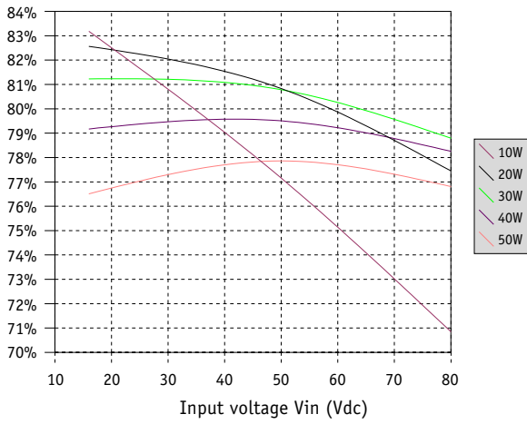
Typical efficiency MGDS750B at 25°C
