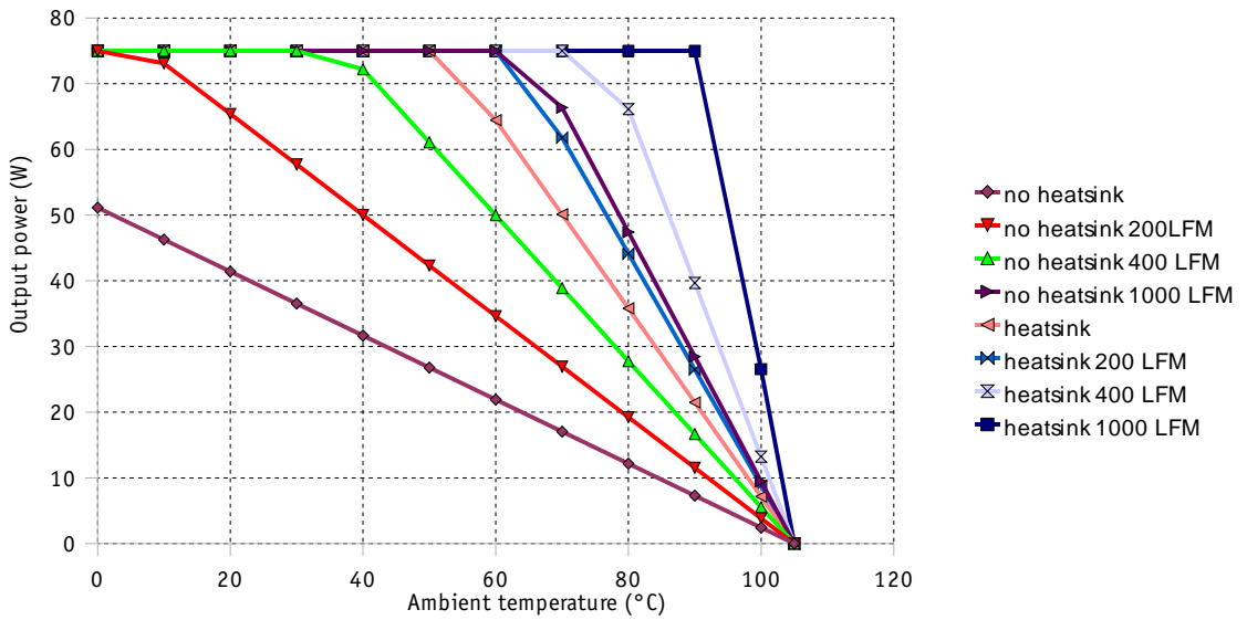
MGDS-75-O-x Series Thermal Curves
