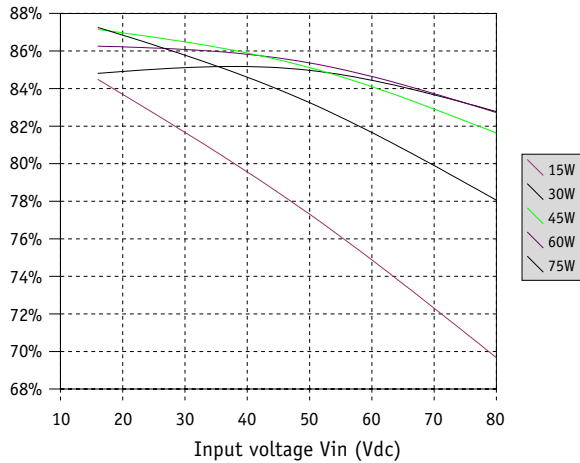
Typical efficiency MGDS750E at 25°C
